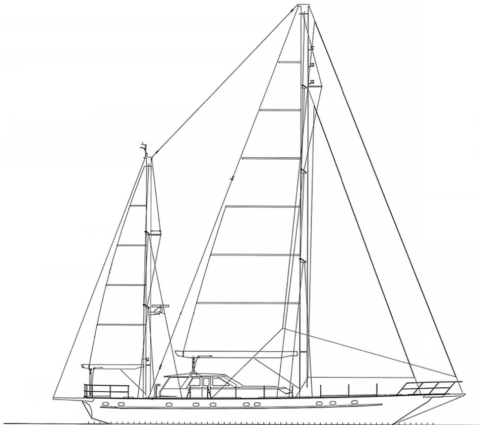
Sailplan
