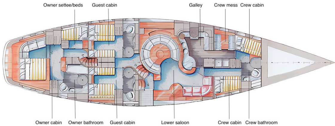
Deck and interior layout
